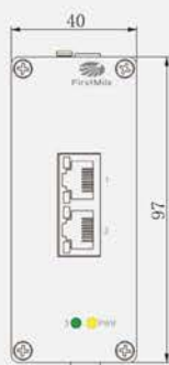
403 Front View
