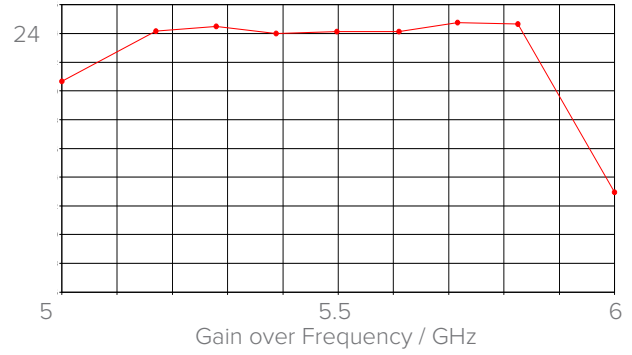
Vertical polarization
