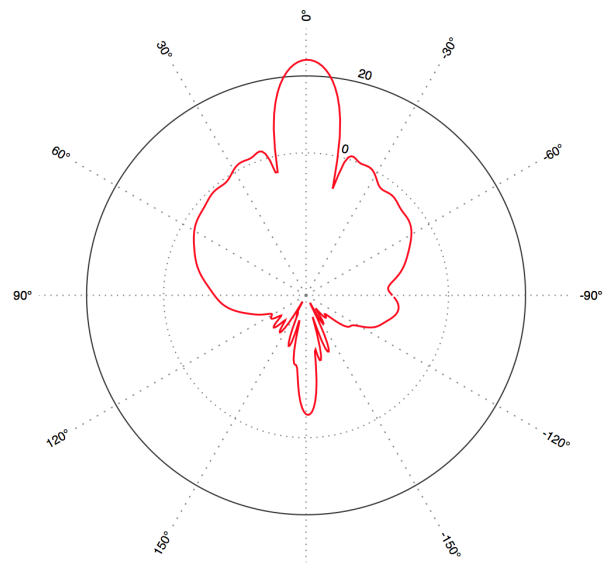
Vertical 90 deg
